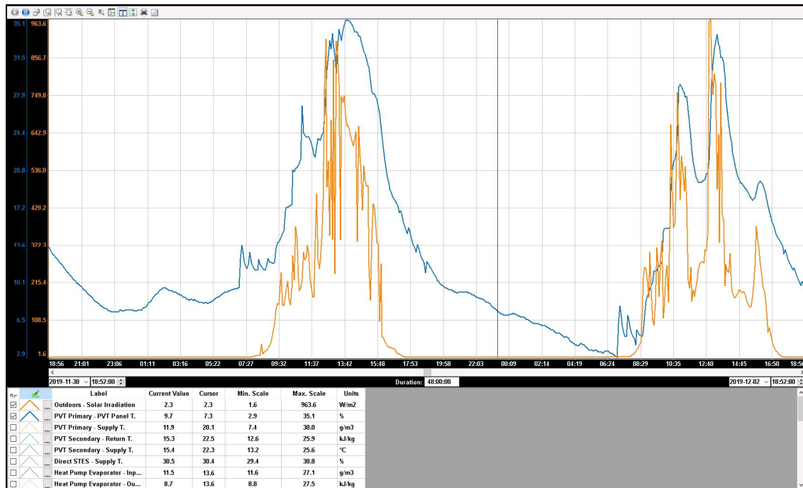
Figure 3.58: Plot of the 'Outdoors - Solar Irradiation' (orange) against the PVT Primary – PV Panel Temperature (blue).
