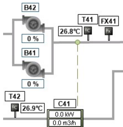
Figure 3.28: Distribution to the customer circuit with its temperature sensors, flow switch, calorimeter, and pumps.
