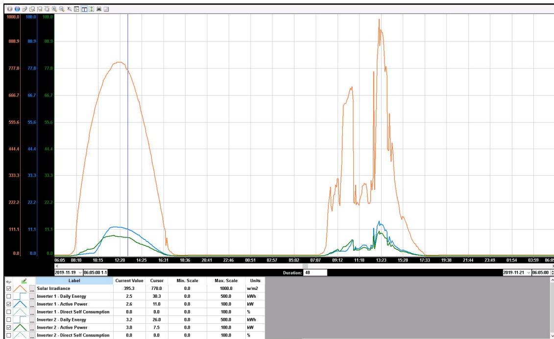
Figure 3.62: The picture shows a plot for 48 hours of 'Solar Irradiance' (orange) and the power output of every FV Inverter (blue and green).
