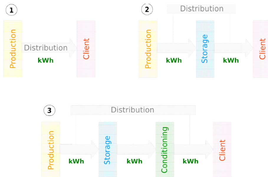
Figure 2.4: The three different energy flows in the CHESS SETUP system.
