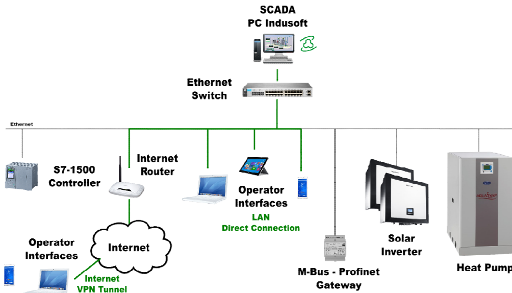
Figure 2.1: CHESS SETUP network architecture.
