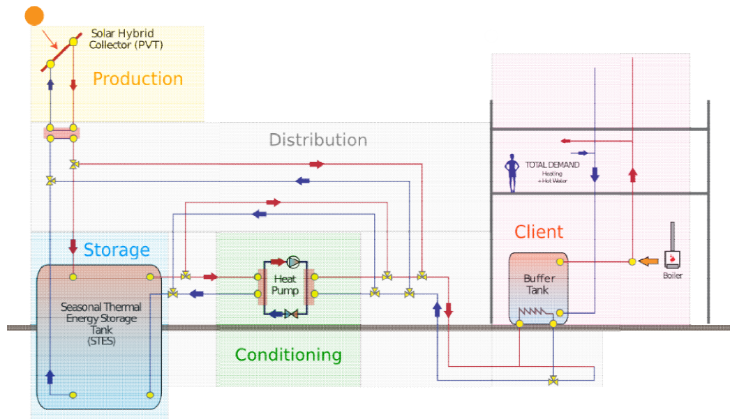
Figure 2.2: Monitoring subsystems in the CHESSE-SETUP project (Deliverable 4.1)
