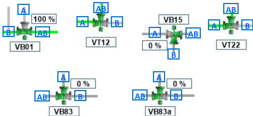
Figure 3.13: Physical positions of the AB, A and B inputs and outputs of the different valves in the CHESS SETUP synoptic.
