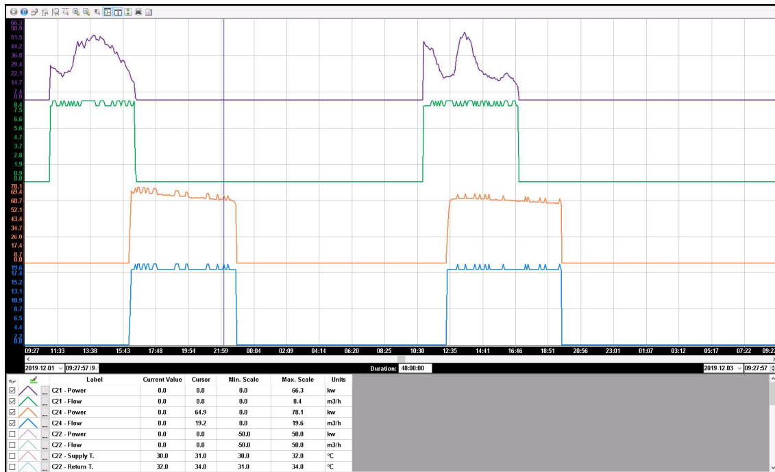
Figure 3.60: plot during 48 hours of the power and flows (in violet and green) for the calorimeter that measures the energy accumulated to the STES (C21) and, in orange and blue, the calorimeter that counts energy extracted from the STES (C24)
