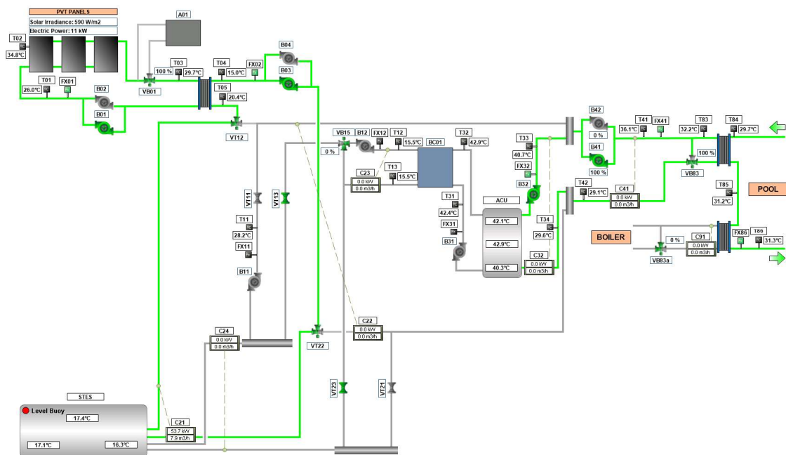
Figure 3.12: Example of the system in Heat Pump Working
