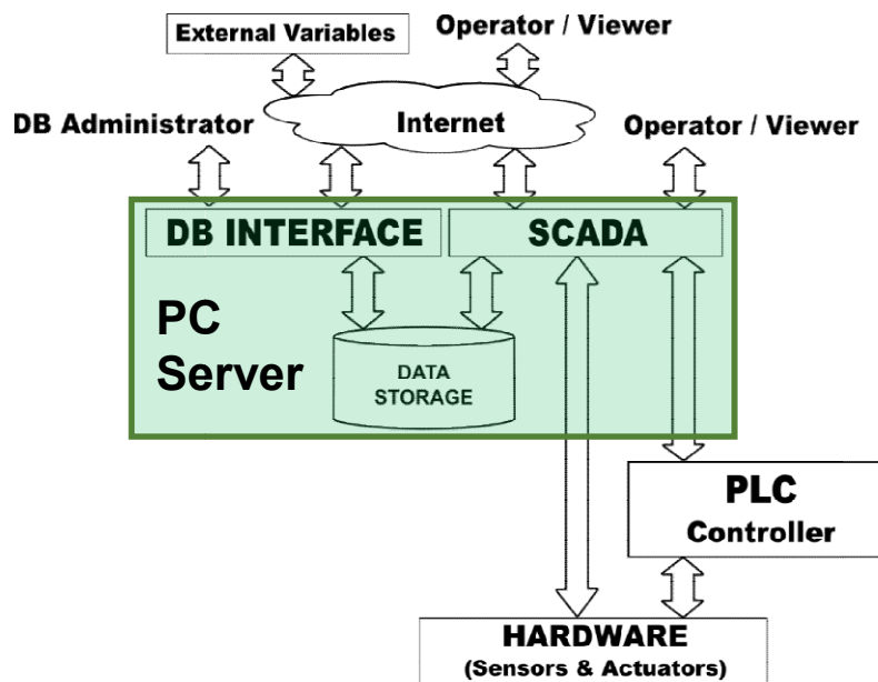
Figure 2.5: Interaction of the different CMS subsystems.
