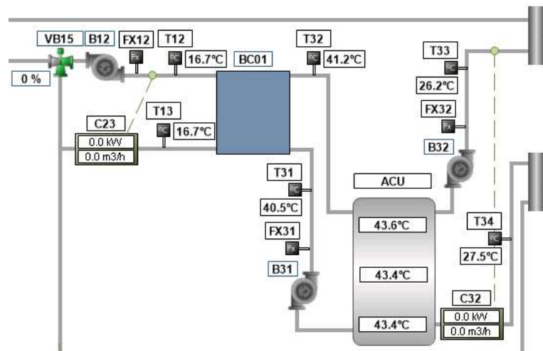
Figure 3.25: Synoptic area for heat pump monitoring and control.
