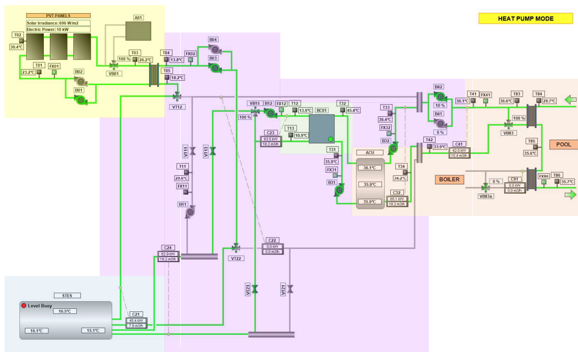
Figure 2.3: Implemented monitoring subsystems in the CHESSE-SETUP project
