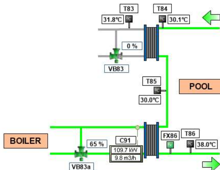
Figure 3.30: Pool exchangers sub-circuit and its elements
