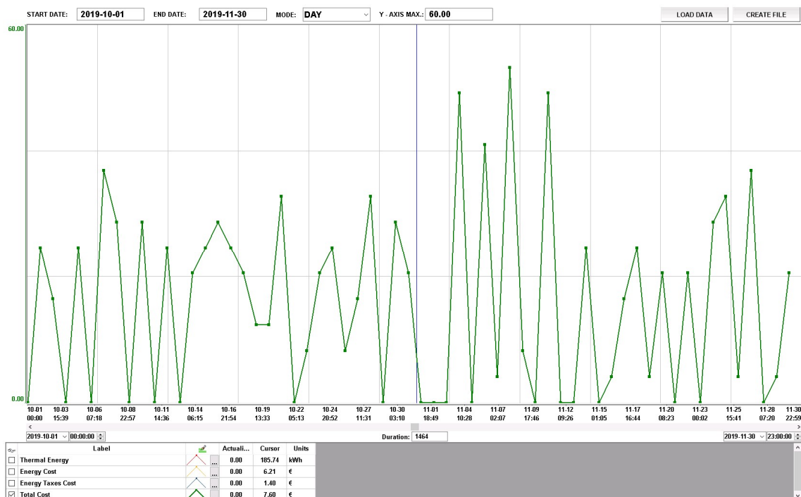
Figure 3.75: The picture shows a plot with the daily thermal savings in € during the period [2019/10/01, 2019/11/30].
