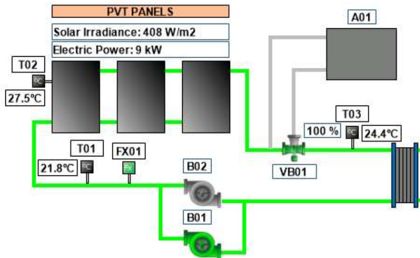
Figure 3.15: PVT primary circuit
