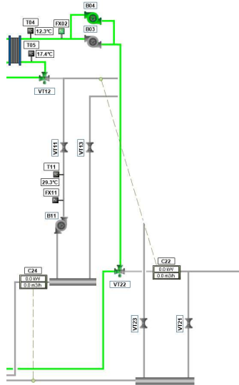
Figure 3.24: Synoptic area referring to the PVT secondary circuit and the STES output to the customer either directly or through the heat pump.
