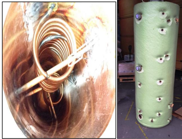
Figure: University of Ulster CST system (Source: University of Ulster)
