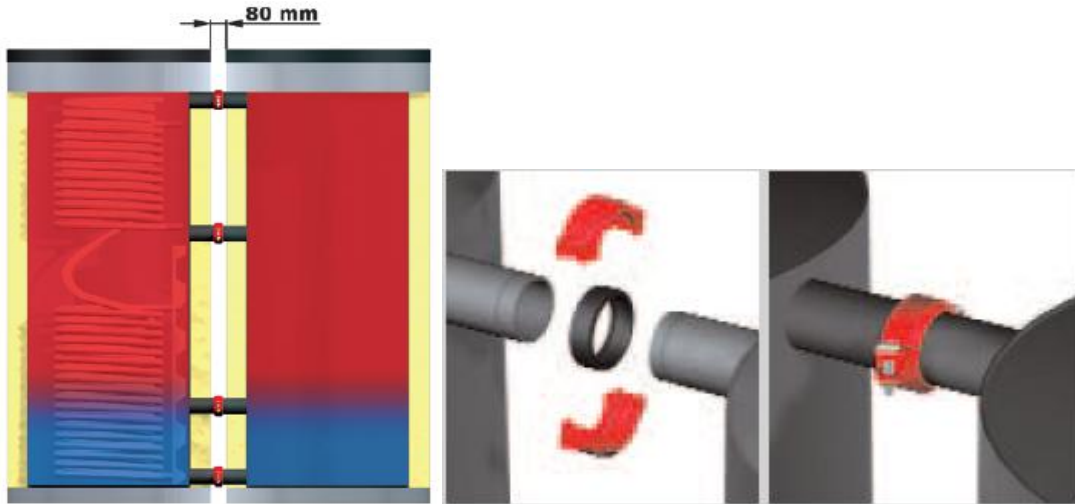
Figure: Connected Stratification tanks (Source: Fröling)
