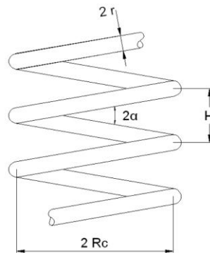
Figure: A Helical Pipe (Source: University of Ulster)
