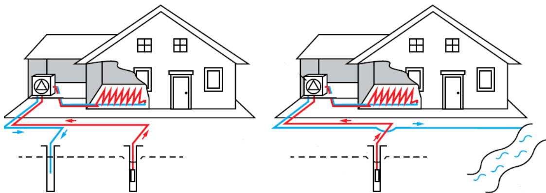
Figure: Open system with heat pump configurations (Source: IDAE Geotermia)
