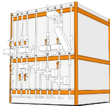
Figure: PU Storage Container (Source: FSAVE, FLEXSAVE Wärmepufferspeicher)
