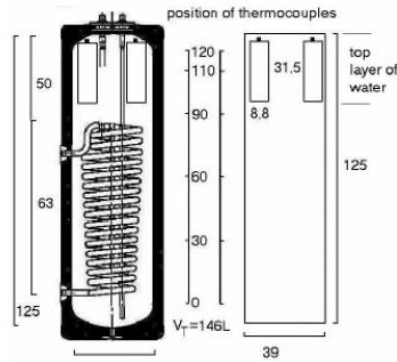
Figure: PCM modules included in domestic hot water tanks (Source: D2.1)
