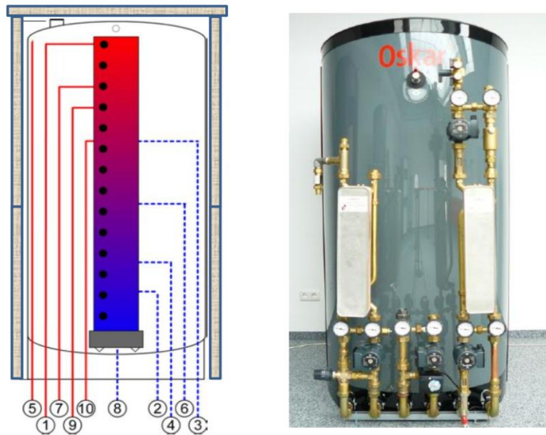
Figure: stratification system of Ratiotherm's Oskar
