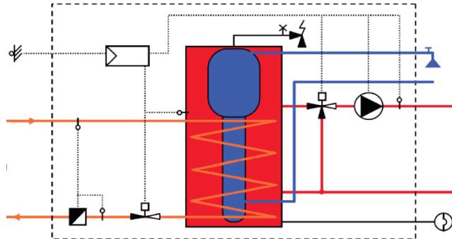
Figures: Steel Tank Design (Source: Haase, SOLUS II Solar-Kombispeicher, Jenni, Swiss Solartank)
