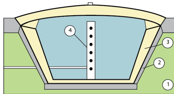
Figure: Pit thermal energy storage (PTES) system.
